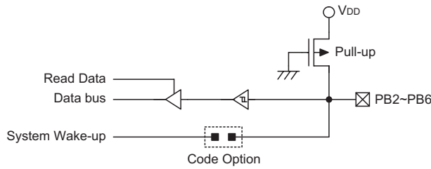
PB2~PB6 Input Lines
