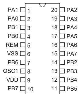
HT48RA0-3/HT48CA0-3 20 SSOP-A
