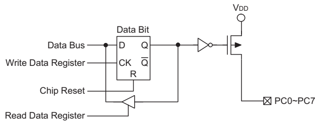
PC Output Port
