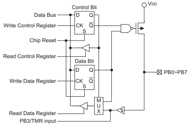
PB Input/Output Port
