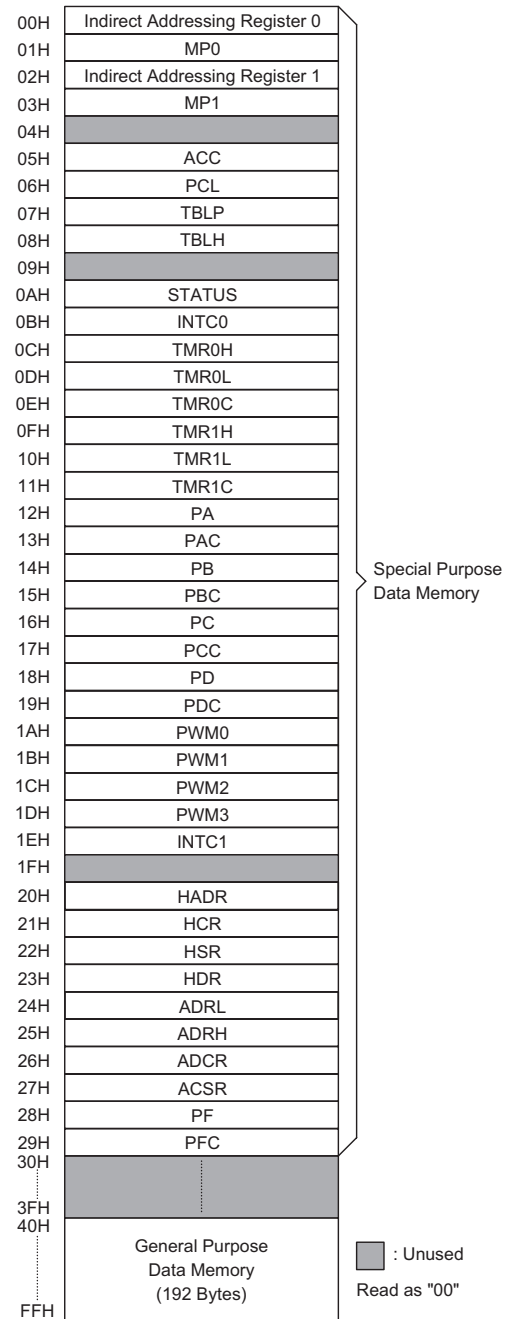
RAM Mapping
