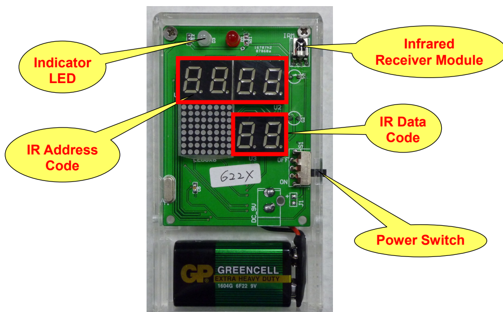
Fig 2 : Infrared Receiver
