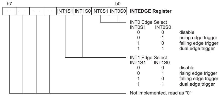
Interrupt Active Edge Register – INTEDEGE
