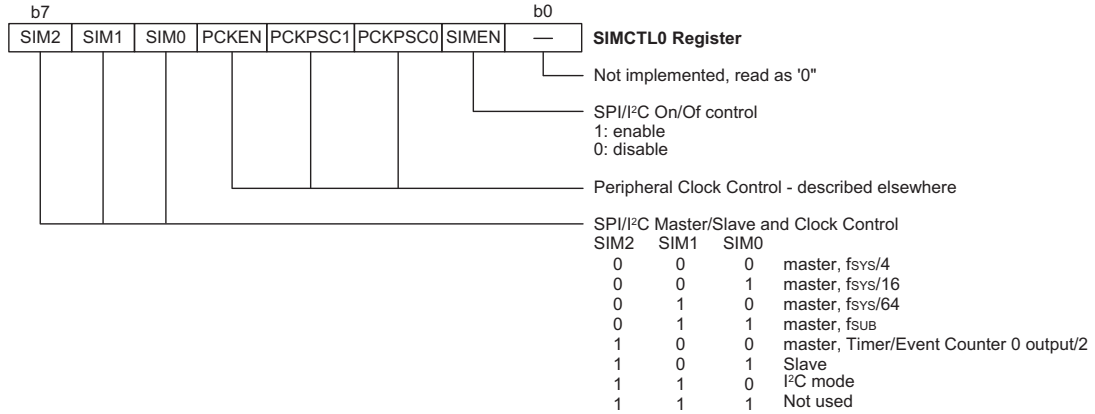
SPI/I²C Control Register – SIMCTL0
