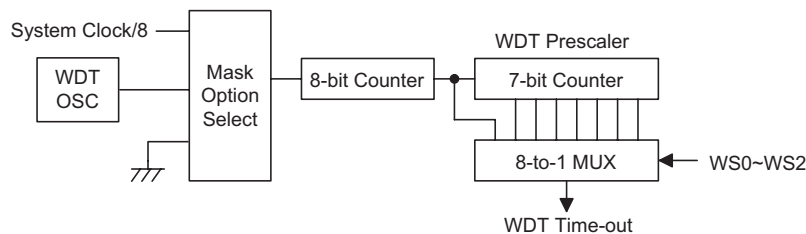
Watchdog Timer
