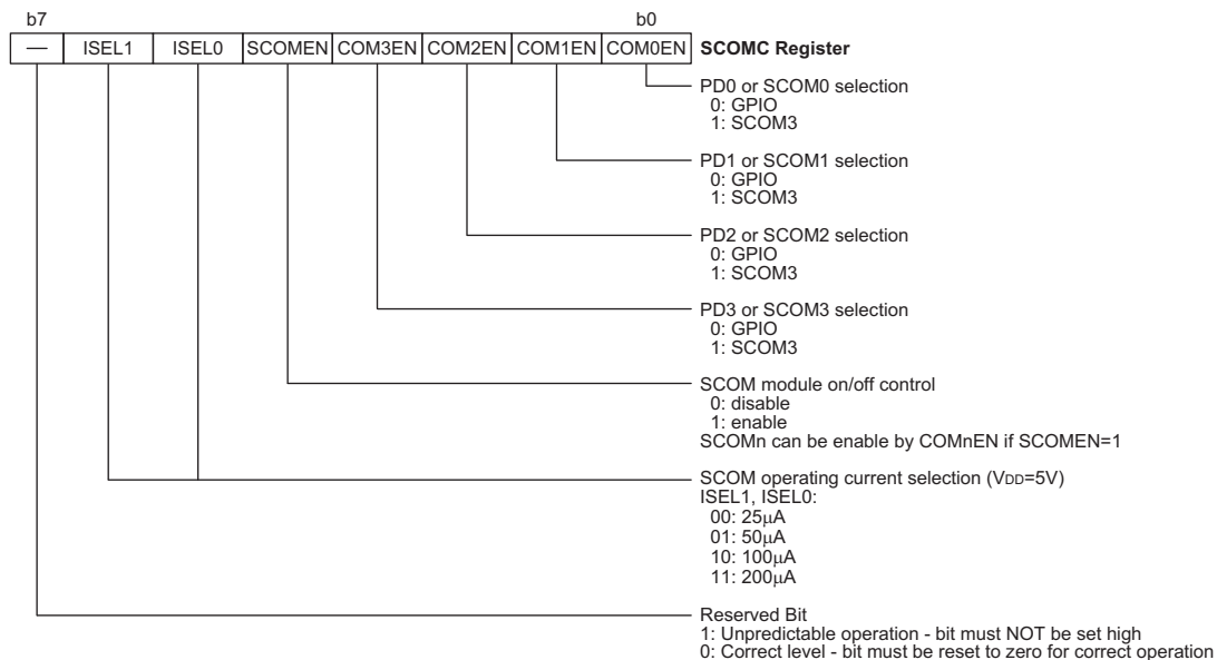
SCOMC Register
